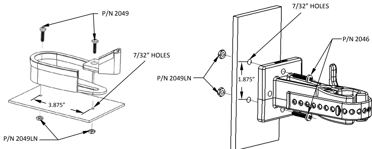
FIGURE 1 (Thru Mounting Method)
