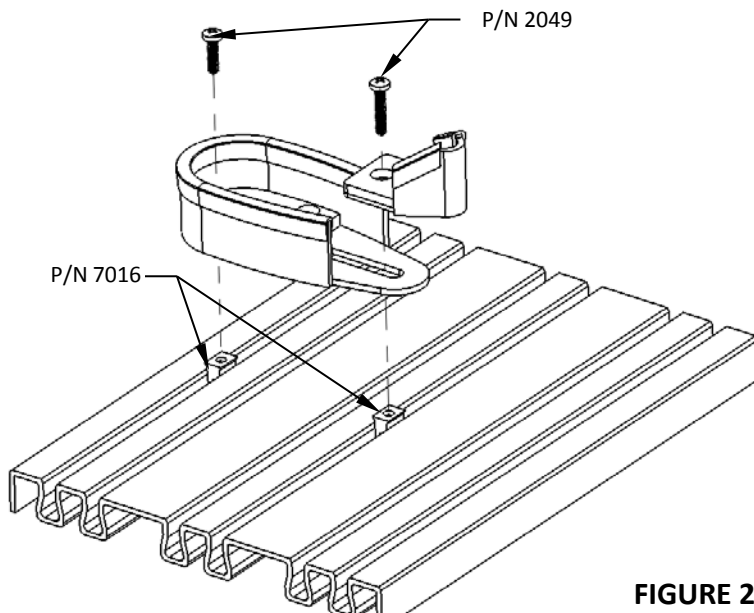
VERTICAL MOUNTING KIT
