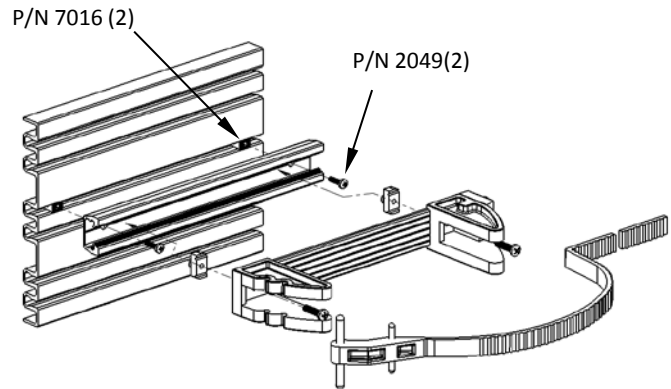
SUPER ADJUSTMENT ATTACHMENT (See INS-K5050 for more installation information)
