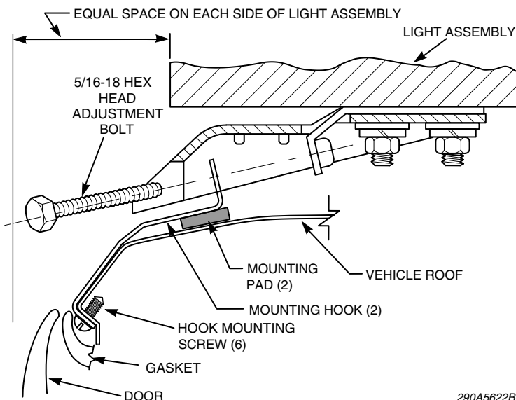
Figure 1 Lightbar attached with hook kit to vehicle
