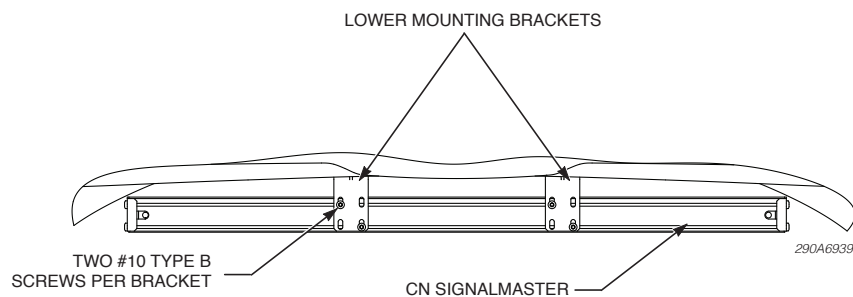
Figure 2 CN SignalMaster mounted to lower bracket assemblies
