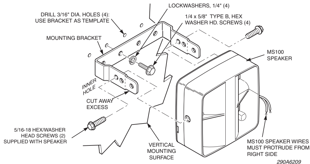
Figure 1: ES100 and MS100 vertically mounted using inner bracket holes
