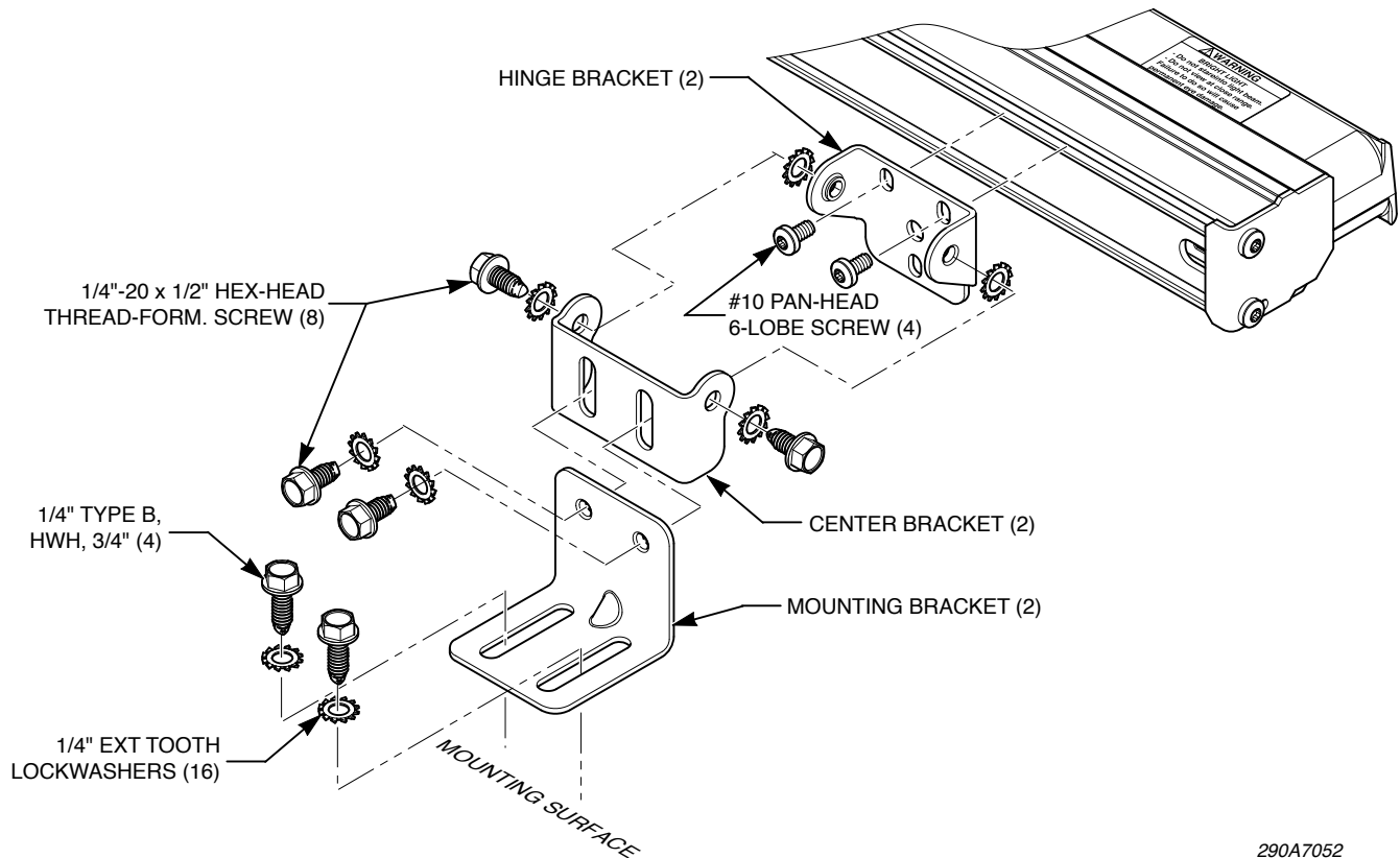
Figure 1 Exploded view of CN SignalMaster attached to mounting surface
