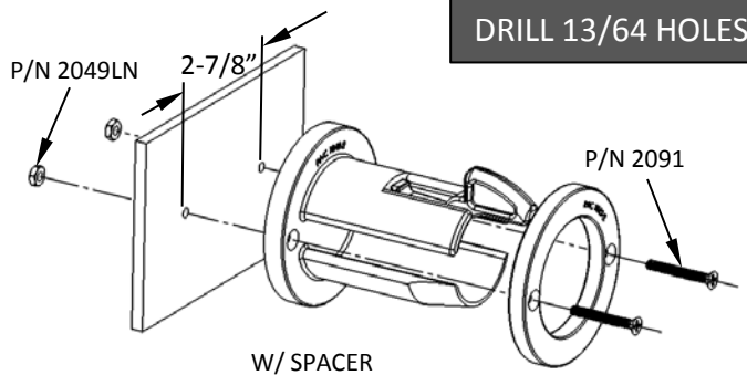
FIGURE 1 (Thru Mounting Method)
