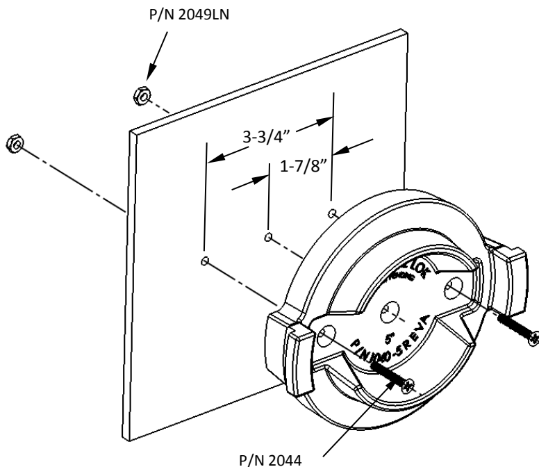
FIGURE 1 (Thru Mounting Method)
