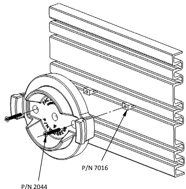
FIGURE 2 (PAC TRAC Mounting)
