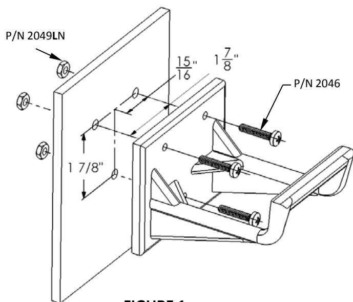
FIGURE 1 (Thru Mounting Method)
