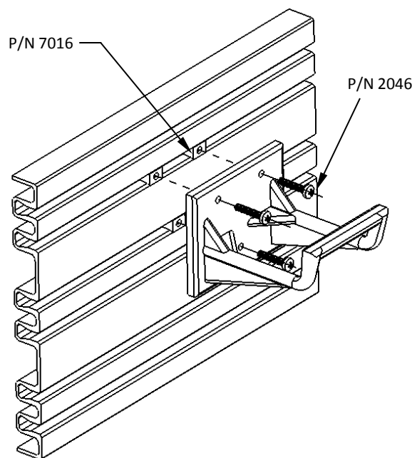
FIGURE 2 (PAC TRAC Mounting)
