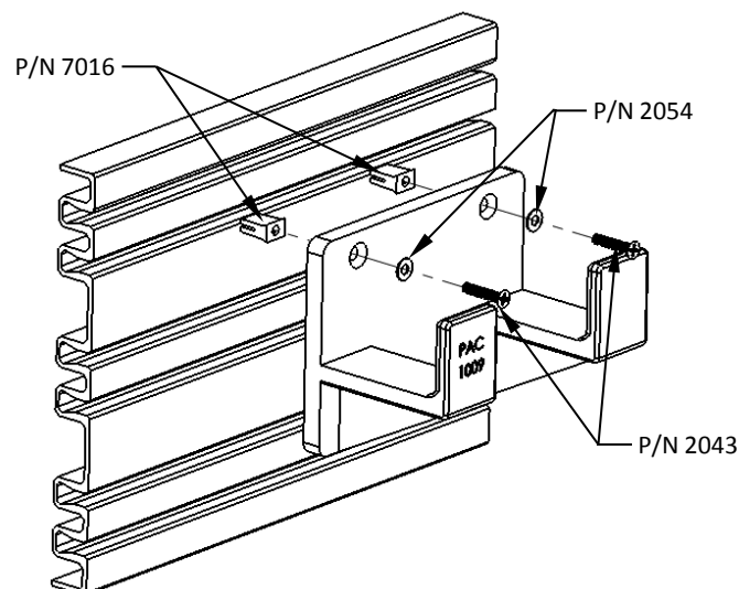
FIGURE 2 (PAC TRAC Mounting)
